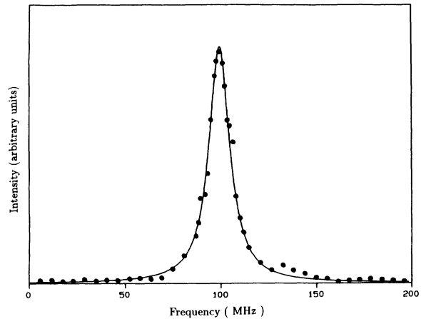
FIG. 2. Example of Lorentzian fit to data. The observed FWHM linewidth of 13 MHz is power broadened from the natural linewidth of 5 MHz. This broadening did not affect the determination of the Stark shift as is discussed in the text.
